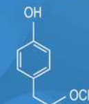
4-(2-METHOXYETHYL) PHENOL
