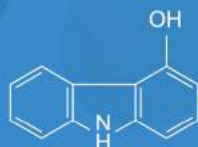
4-HYDROXY CARBAZOLE
