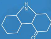
1,2,3,9-TETRAHYDRO-4(H) -CARBAZOL-4-ONE
