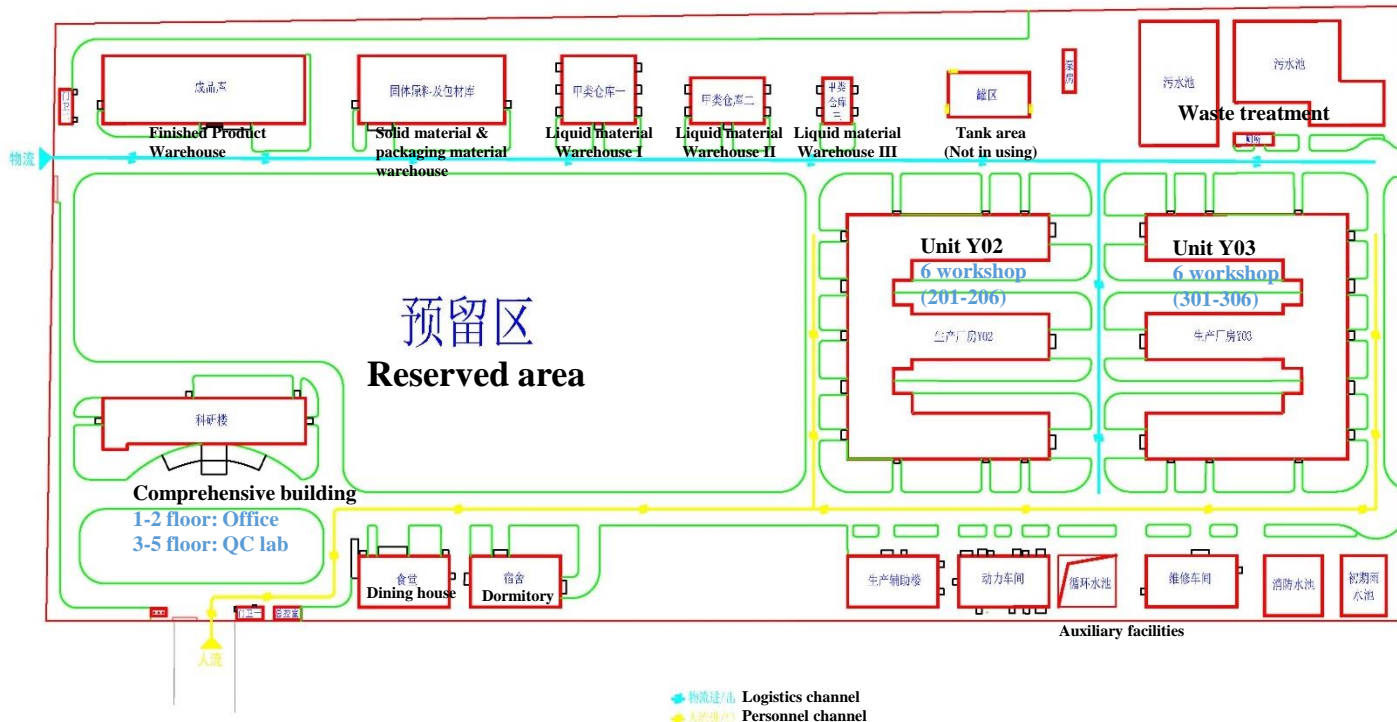
The layout of Yucheng Manufacturing Base
