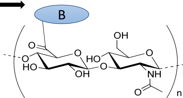
Hyaluronic acid derivative B
