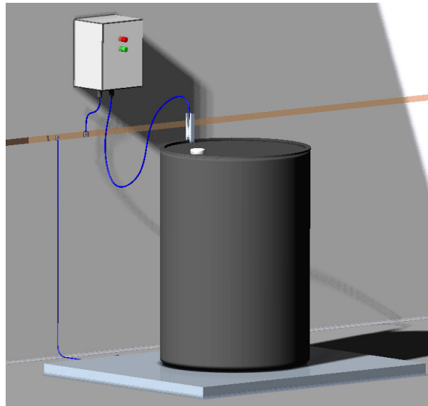
Example of correct grounding technique for a static dissipative drum
